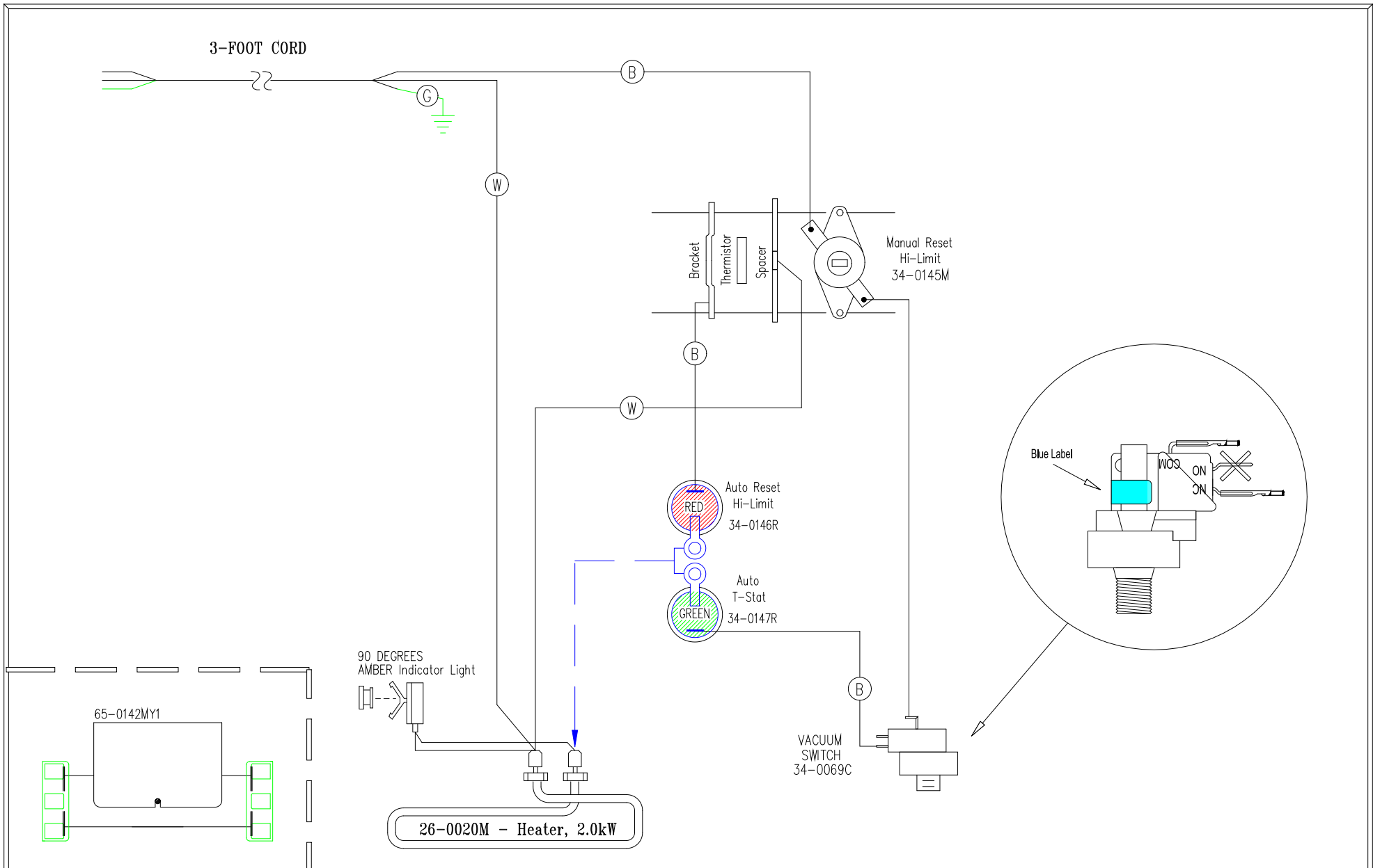
Wiring Diagram, Bath, Depicting New Solderless Wiring
